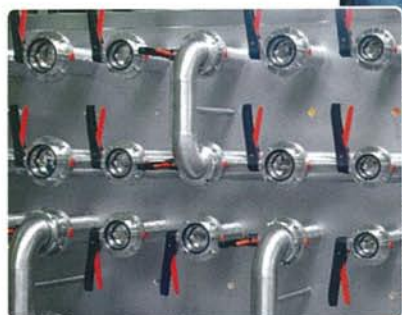
Valves and pipework – Kieselmann specialties and a typical tank top with its cover removed.
